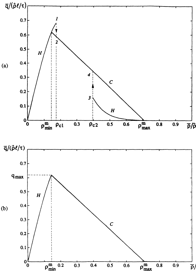
FIG. 12. The average fundamental diagram for a circular road of a large enough circumference L . The curves H correspond to the homogeneous time-independent state of traffic flow, the line C corresponds to the states of traffic flow with one or more wide stationary moving clusters (or anticlusters).
