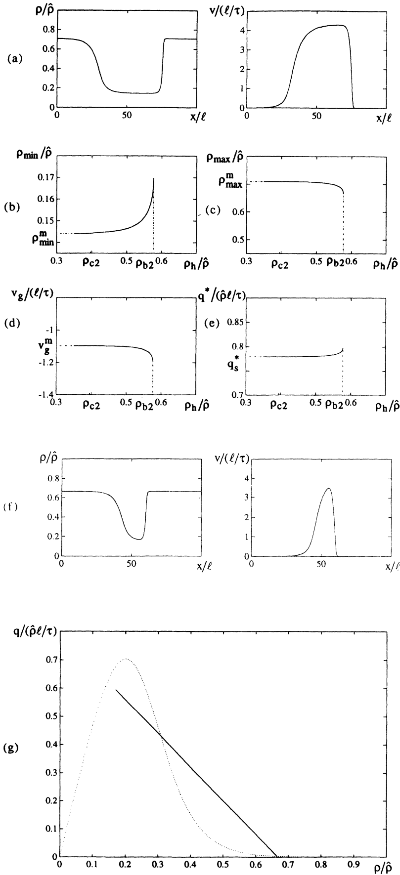
FIG. 11. The “anticlusters” in traffic flow: (a) the distributions \rho(x) and v(x) in a wide anticluster, (b)–(e) the dependencies of the minimal density \rho_{\min}^m (b), the maximal density \rho_{\max}^m (c), the velocity v_g (d), and the parameter q^* (e) for anticlusters on \rho_h . In (f) and (g) the distributions \rho(x) and v(x) (f) and the curve q(\rho) (g) for the narrow anticluster for \rho_h = 0.5765\hat{\rho} are shown. L = 100l . The other parameters are the same as in Fig. 1. Dotted line in (g) represents the fundamental diagram from (b). The found boundary value of density for L = 100l is \rho_{b2} \cong 0.5766\hat{\rho} .
